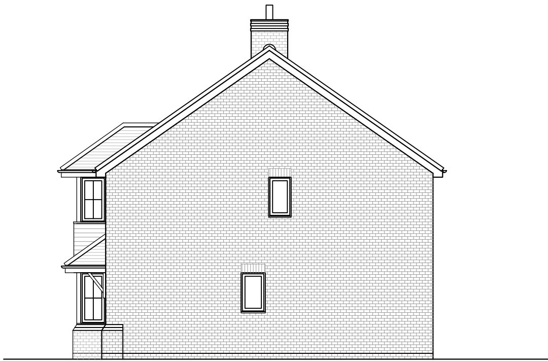
West (Side) Elevation - As Existing
