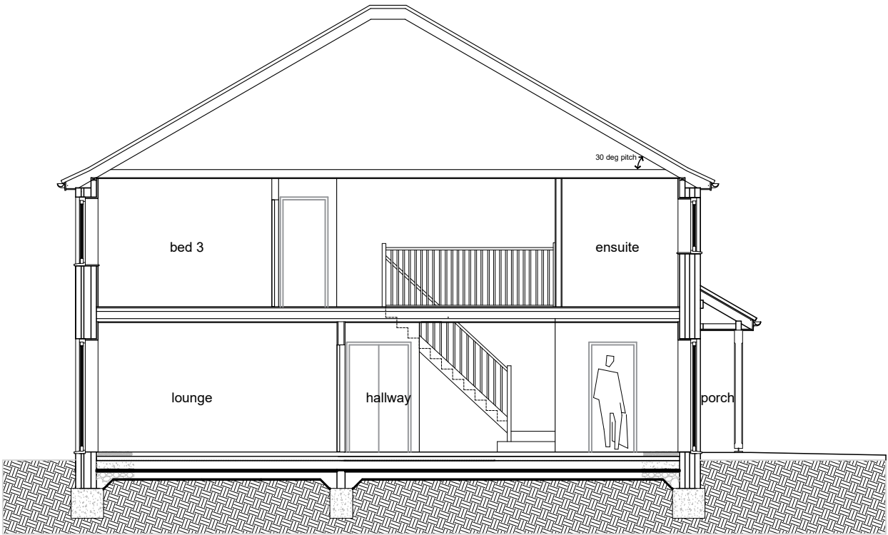
Typical section AA
