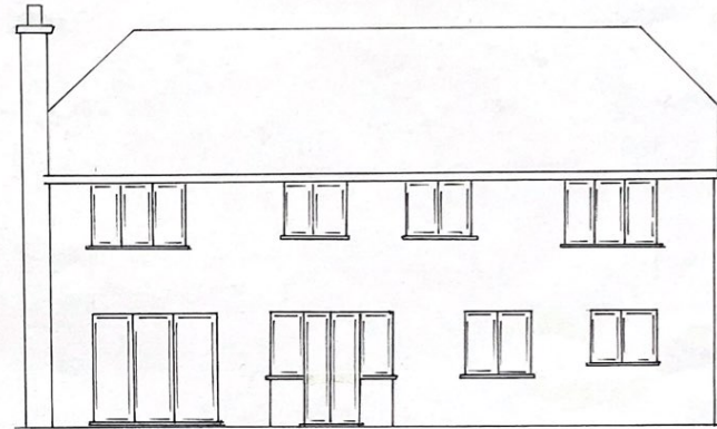
REAR ELEVATION
