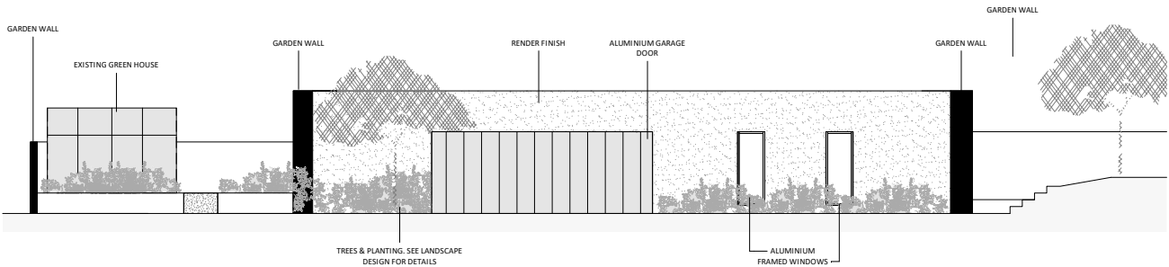
PROPOSED GARAGE FRONT ELEVATION
