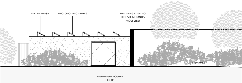
PROPOSED GARAGE SIDE ELEVATION 01
