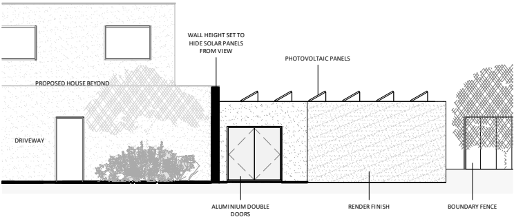
PROPOSED GARAGE SIDE ELEVATION 01
