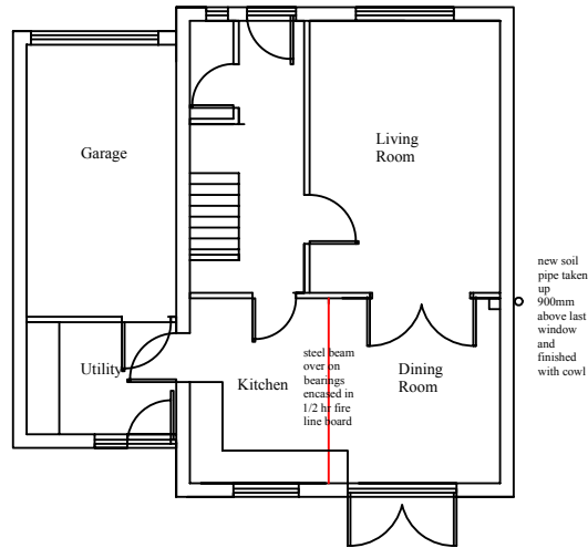
Ground Floor Plan as Proposed
