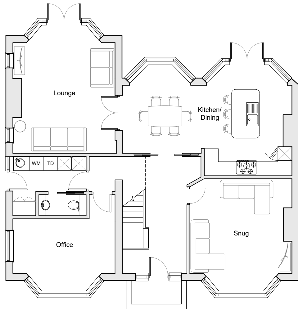
Extant Ground Floor - 1:100
