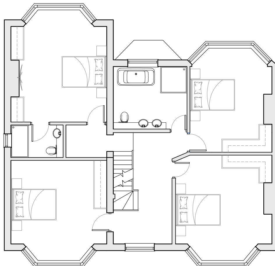
Extant First Floor - 1:100
