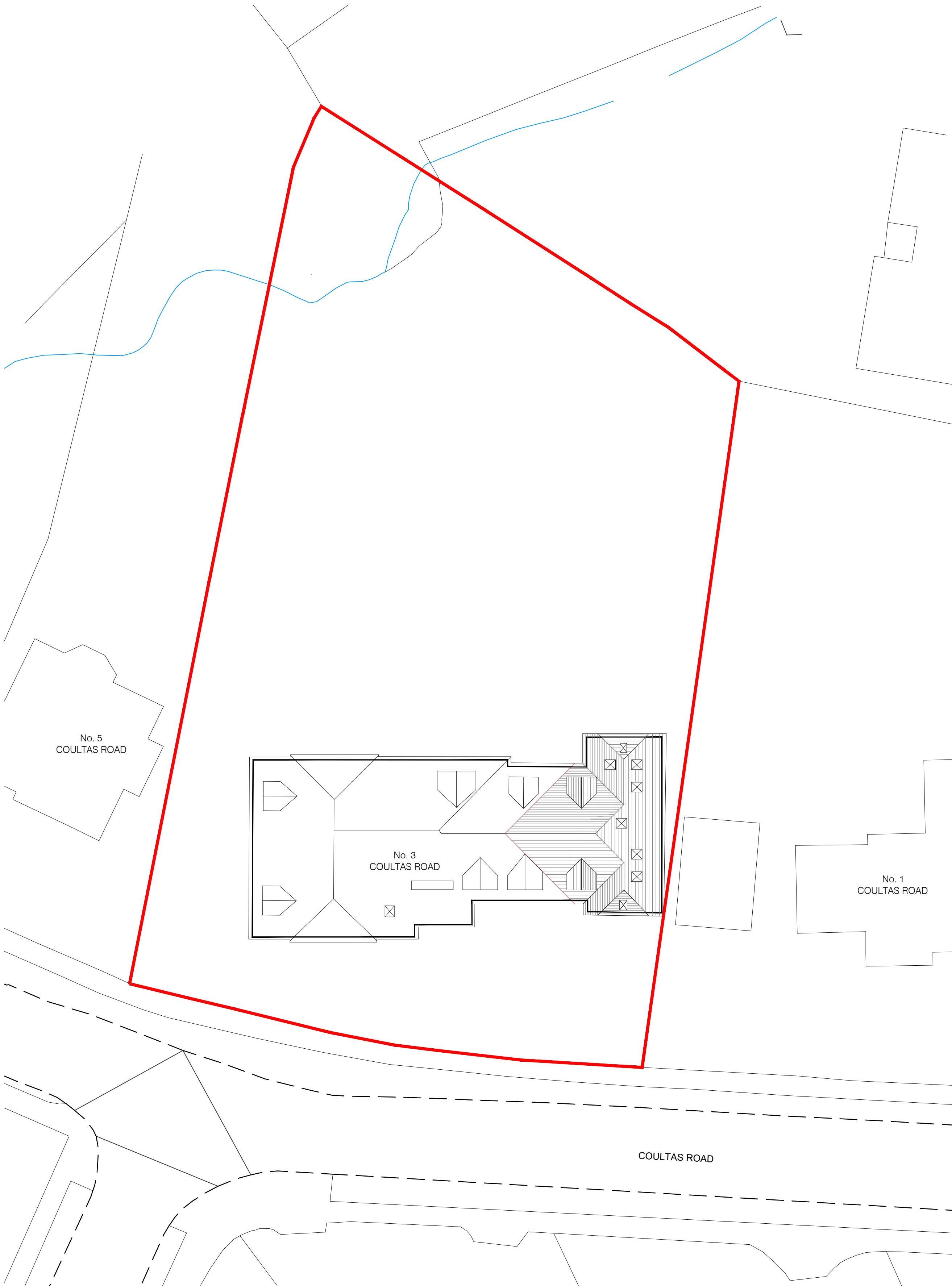
Block Plan - As Proposed Scale 1:200
