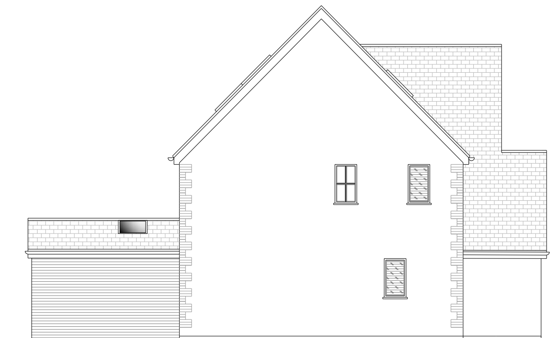
Proposed Left Elevation
