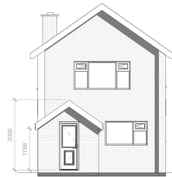
Proposed Elevation-Front
