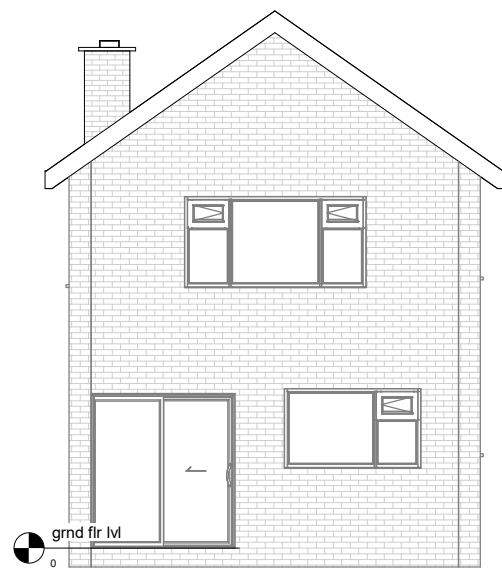
Existing Elevation-Front
