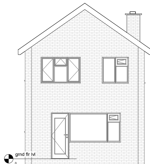
Existing Elevation-Rear
