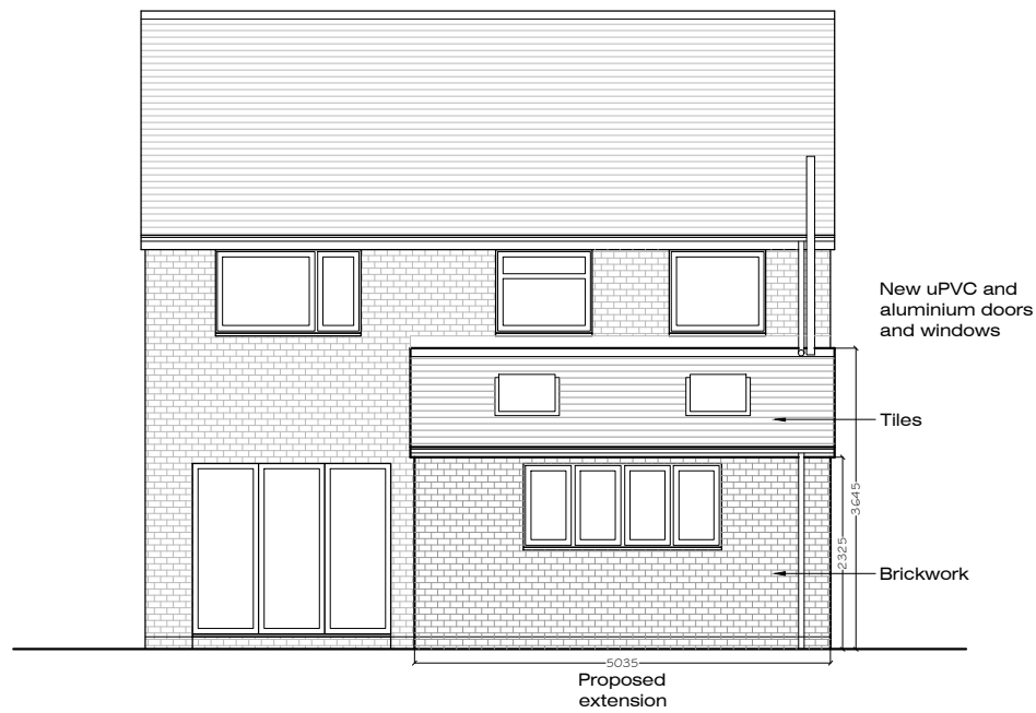
South-West (Rear) Elevation - As Proposed
