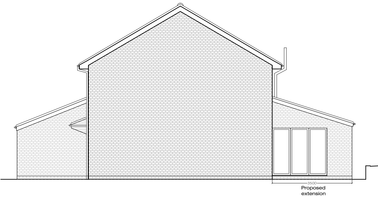
North-West (Side) Elevation - As Proposed
