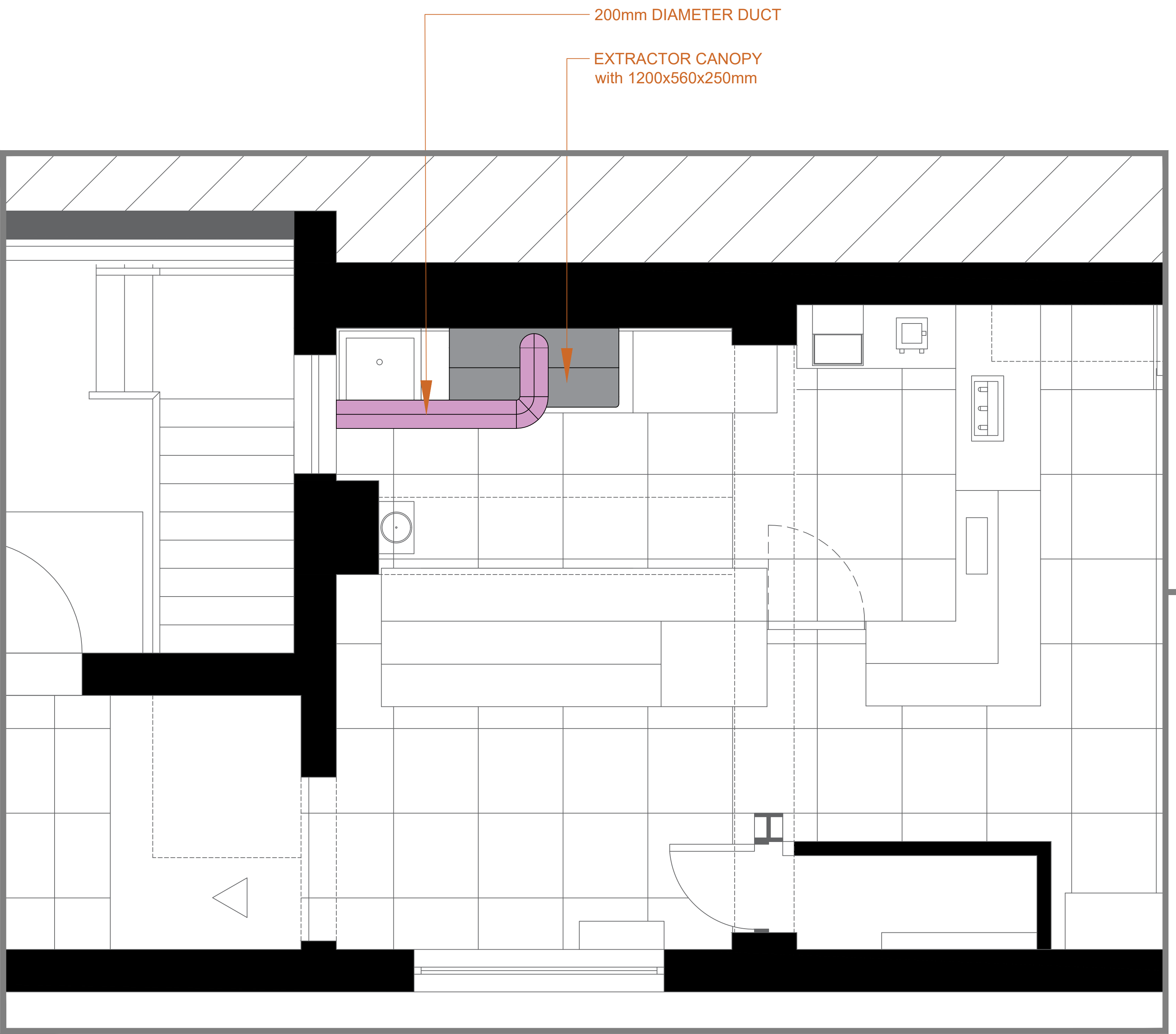
Preparation Zone Scale: 1:20
