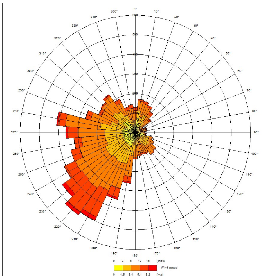
Wind Rose –Southampton Airport
