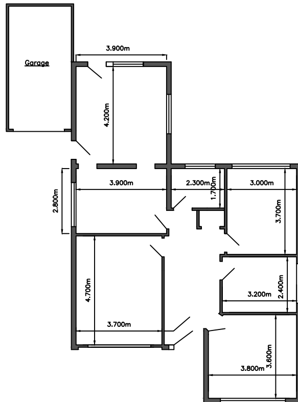
existing ground floor
