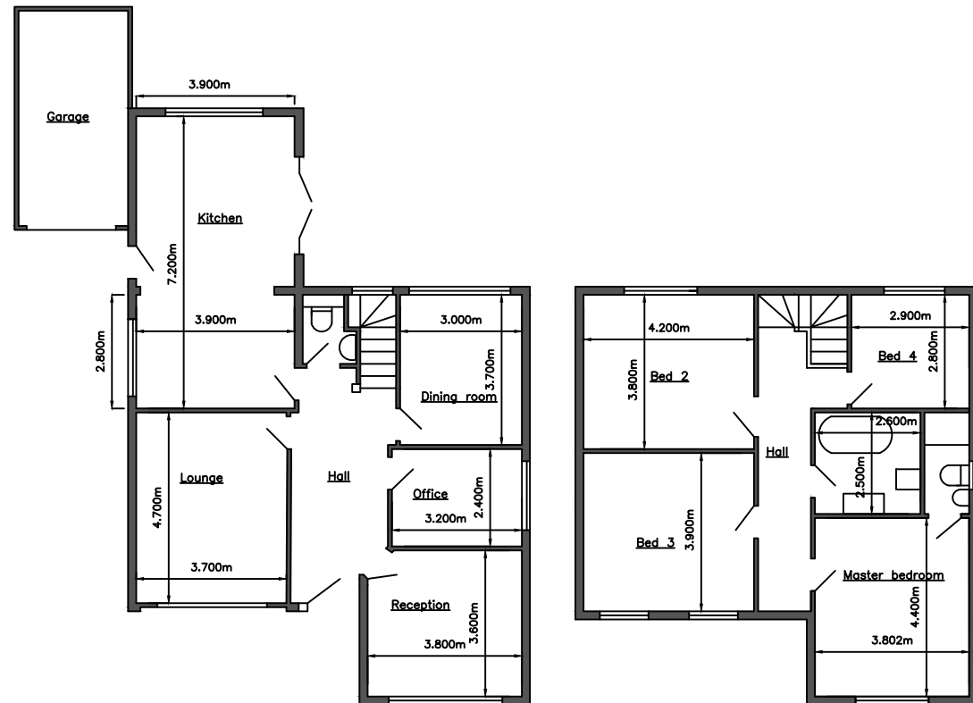
Proposed ground & first floor
