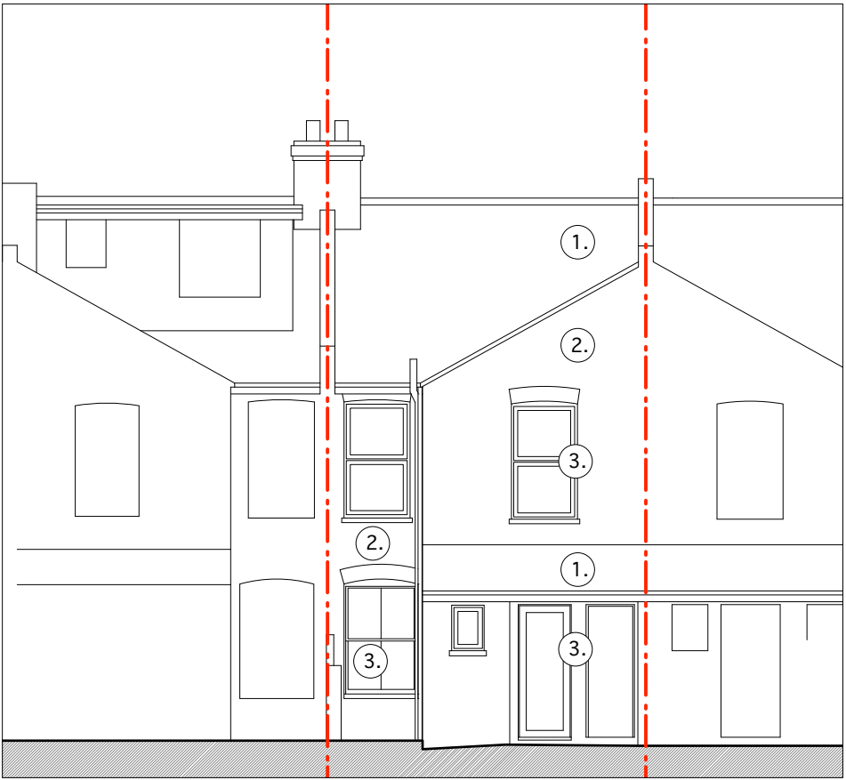
Existing rear / west elevation.
