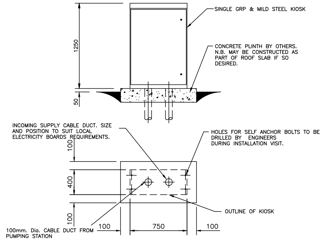
DETAIL OF SINGLE MILD STEEL & GRP KIOSK
