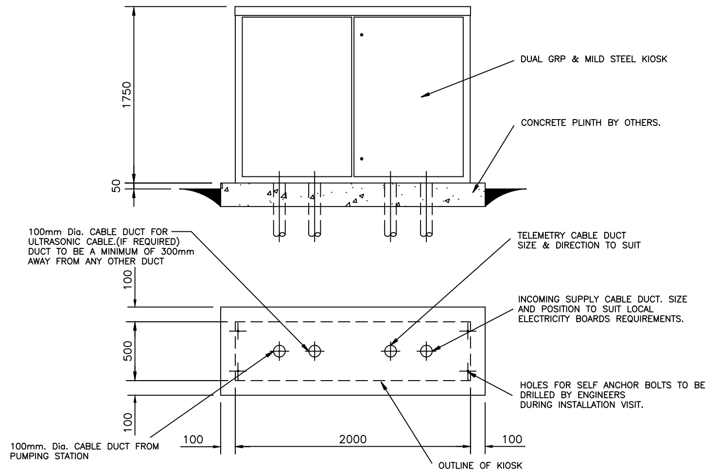
DETAIL OF DUAL MILD STEEL & GRP NWC TYPE KIOSK
