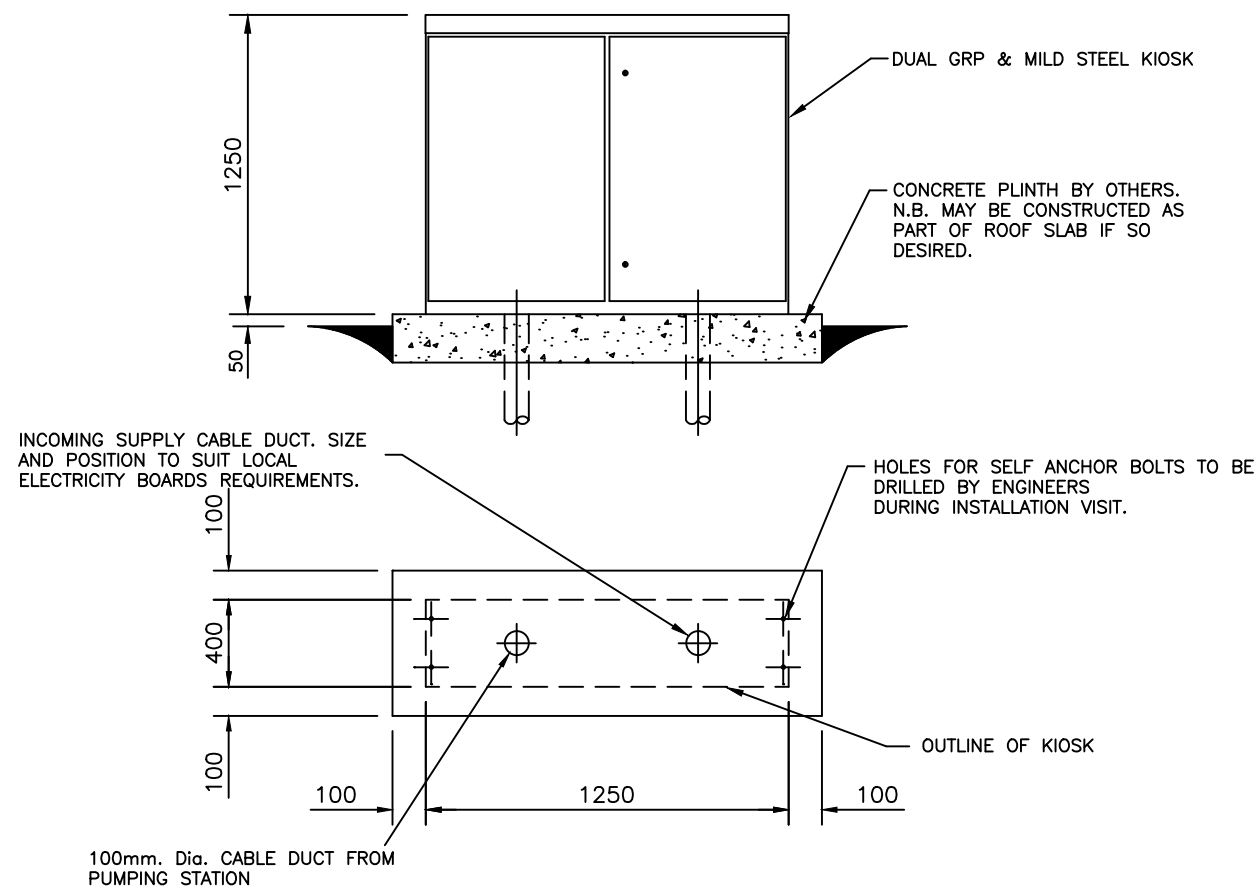
DETAIL OF DUAL MILD STEEL & GRP KIOSK
