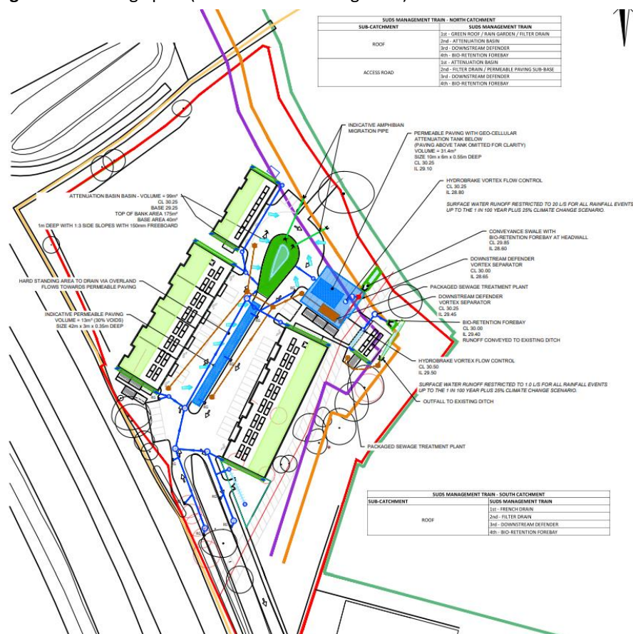
Figure 35. Drainage plan (Fernbrook consulting 2023).
