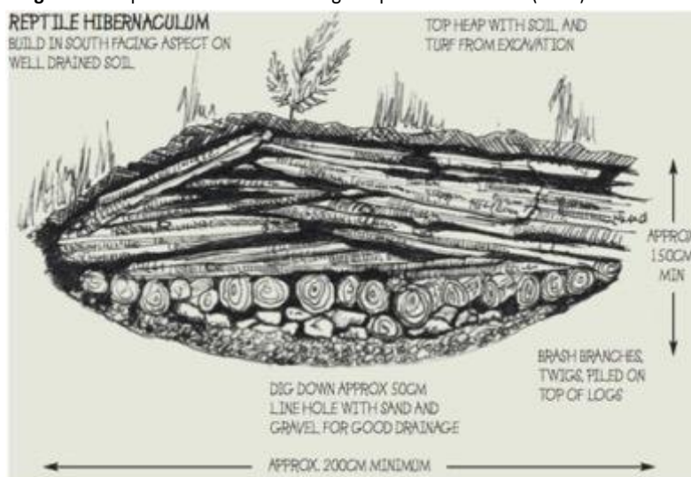
Figure 37. Reptile hibernaculum design as provided in HART (2009).
