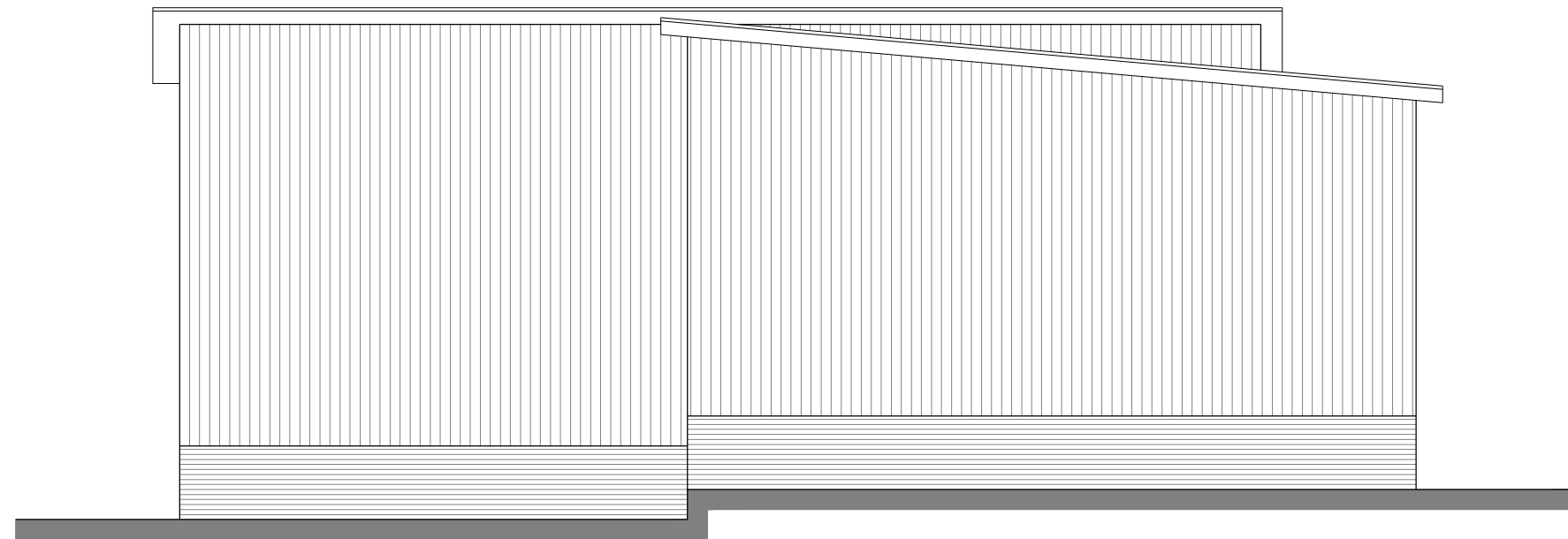
West Elevation
