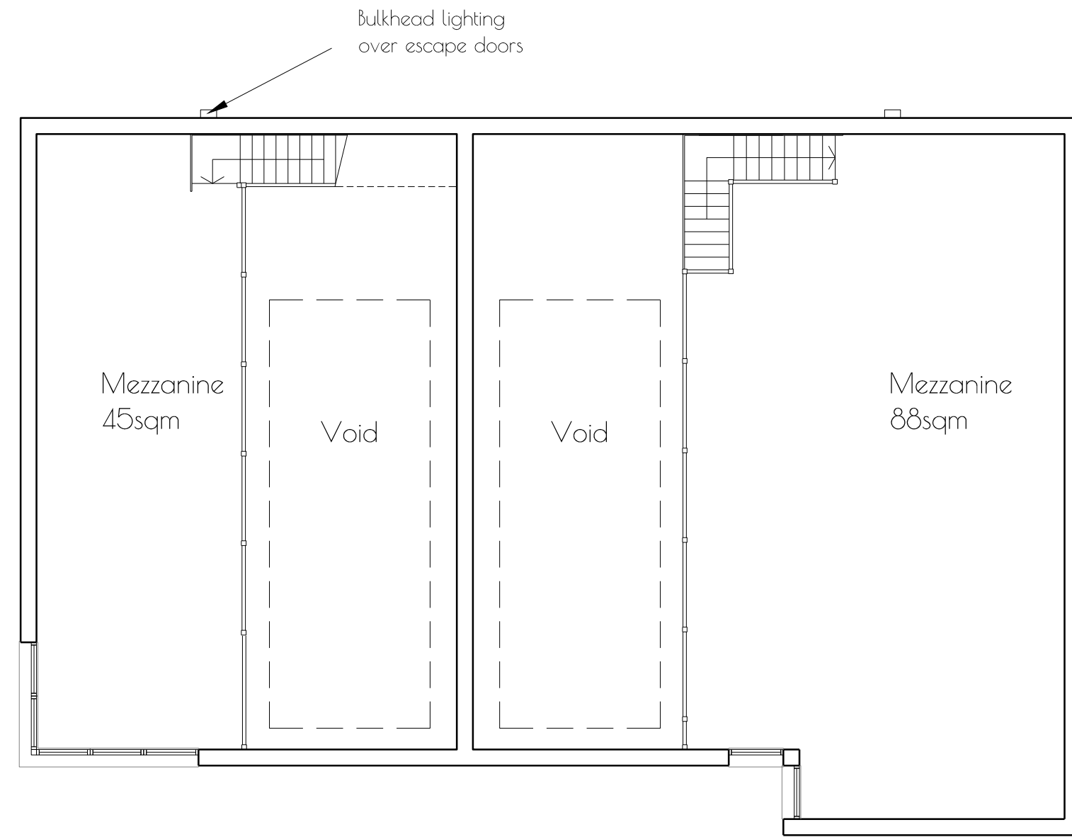
First Floor
