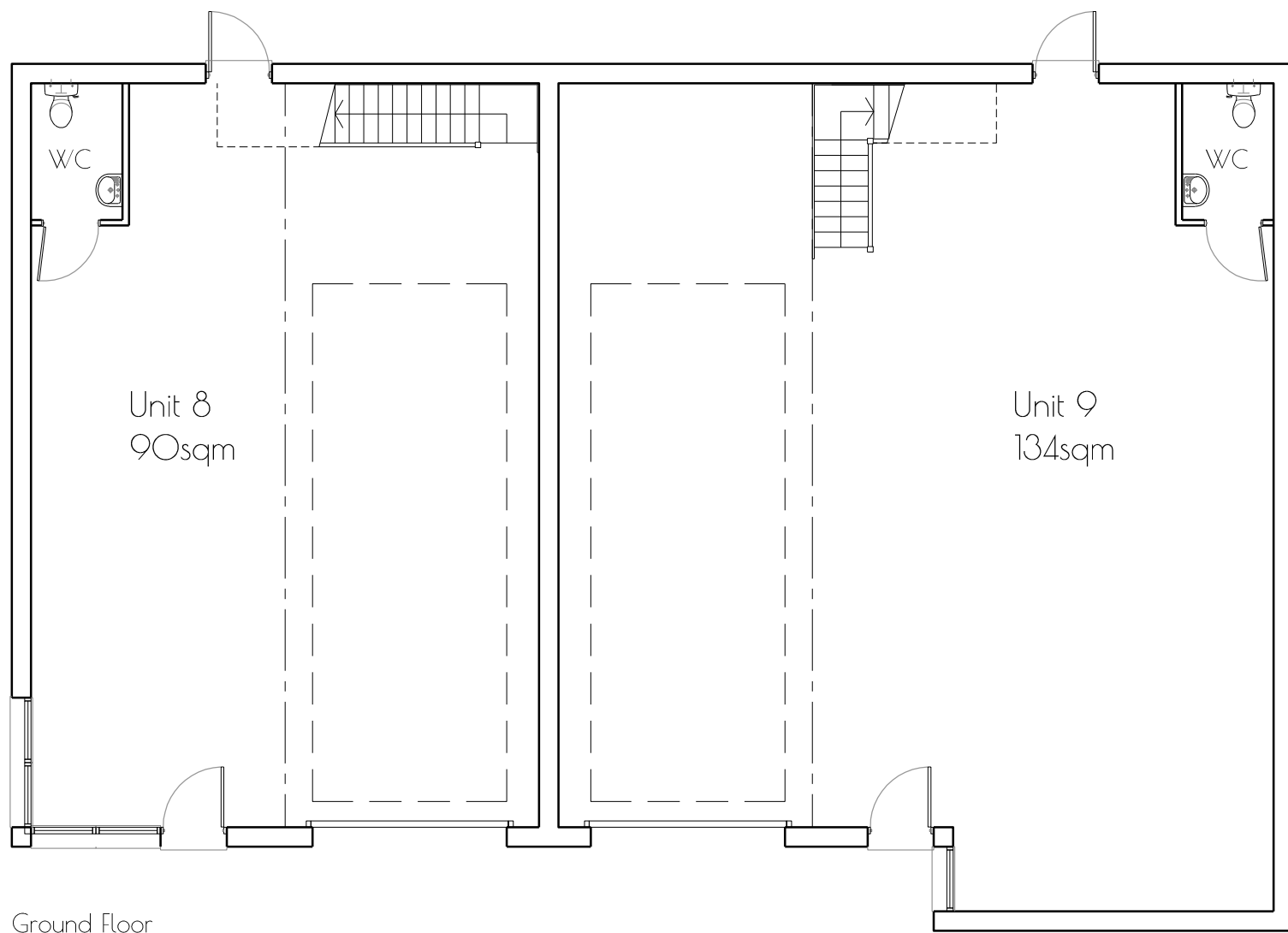
Ground Floor
