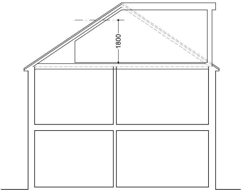
SECTION 1:100
