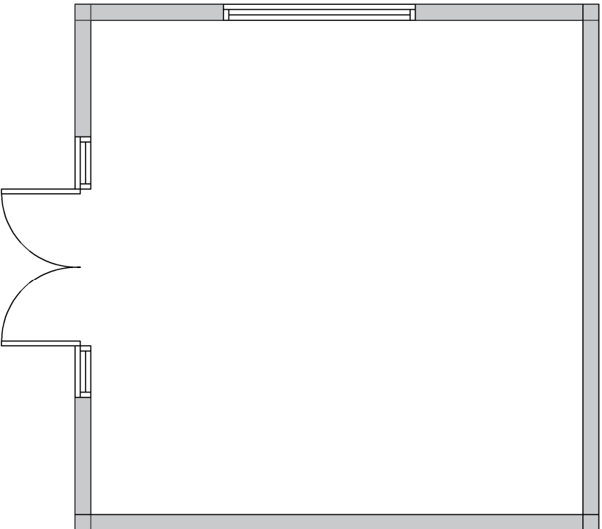
FLOOR PLAN 1:50
