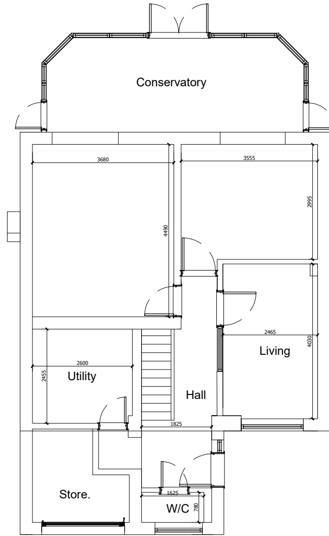
Existing Ground Floor Plan scale: 1:50 @ A1, and 1:100 @ A3
