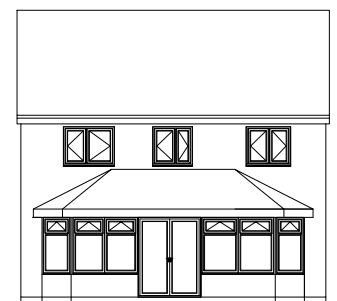
Existing Rear Elevation scale: 1:100 @ A1, and 1:200 @ A3
