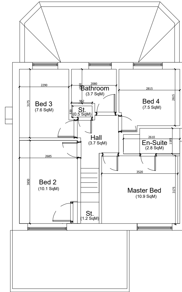
Existing First Floor Plan (48 SqM) scale: 1:50 @ A1, and 1:100 @ A3
