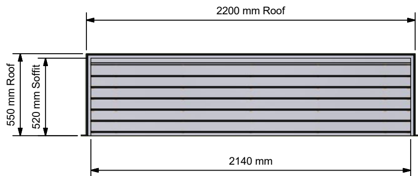
Reflected Plan Elevation ( 1 : 25 )
