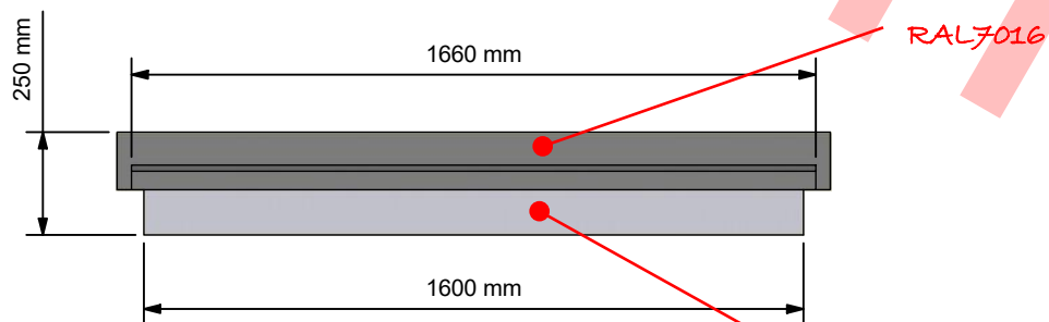
Front Elevation ( 1 : 20 )
