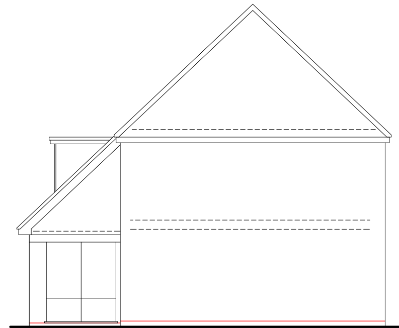
PROPOSED SIDE (WEST) ELEVATION
