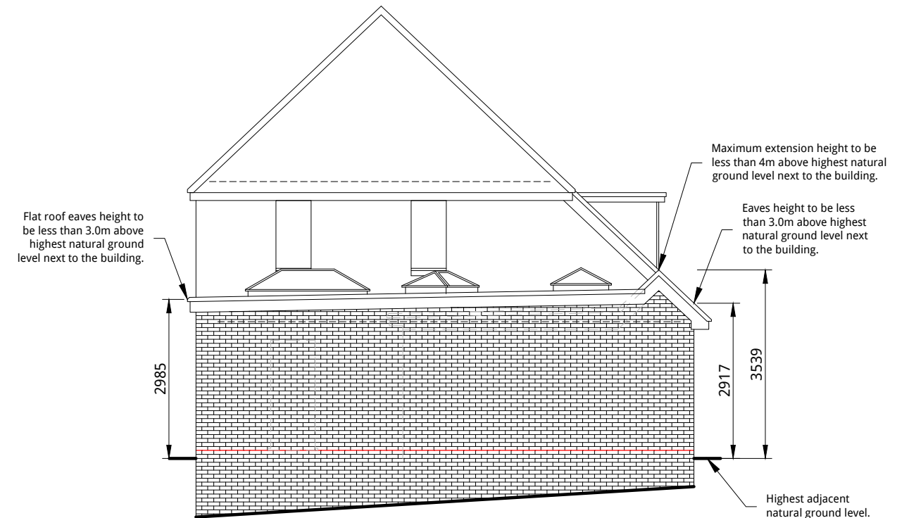
PROPOSED SIDE (EAST) ELEVATION
