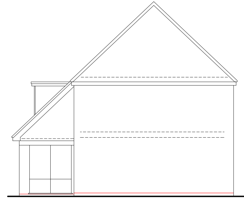
EXISTING SIDE (WEST) ELEVATION
