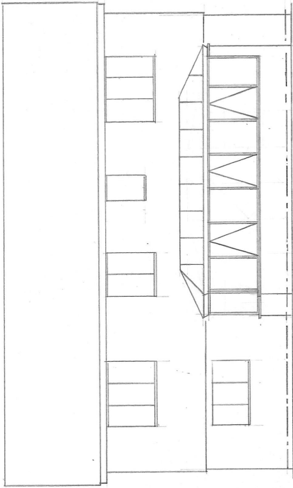
PROPOSED EAST ELEVATION (REAR)
