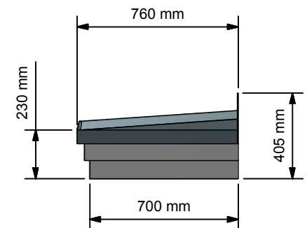
Side Elevation ( 1:25 )
