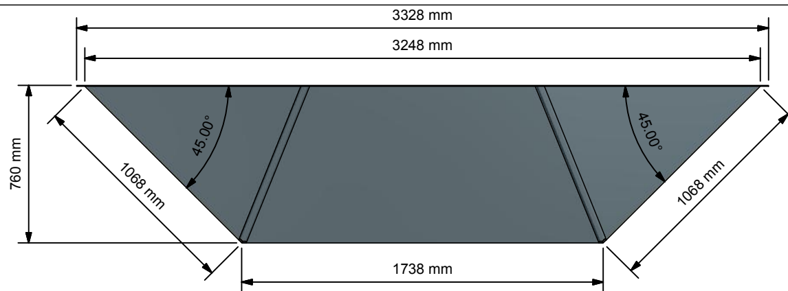
Plan View ( 1:25 )
