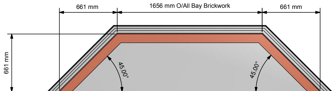
Reflected Plan View Showing Bay Structure Below ( 1:25 )
