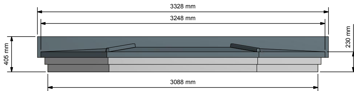
Front Elevation ( 1:25 )
