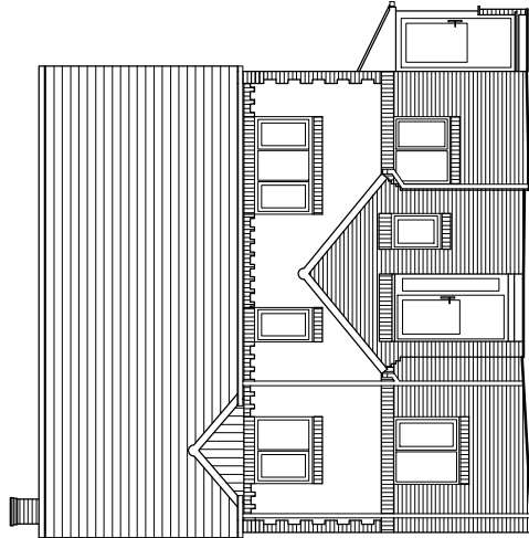
EXISTING NORTH WEST ELEVATION
