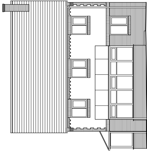
EXISTING SOUTH EAST ELEVATION
