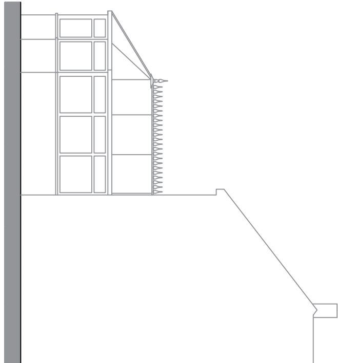
Existing Side Elevation 1:100 @ A3
