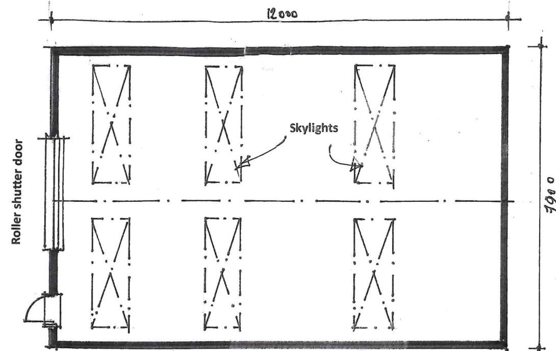
FLOOR PLAN
