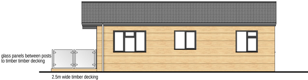
PROPOSED SIDE ELEVATION
