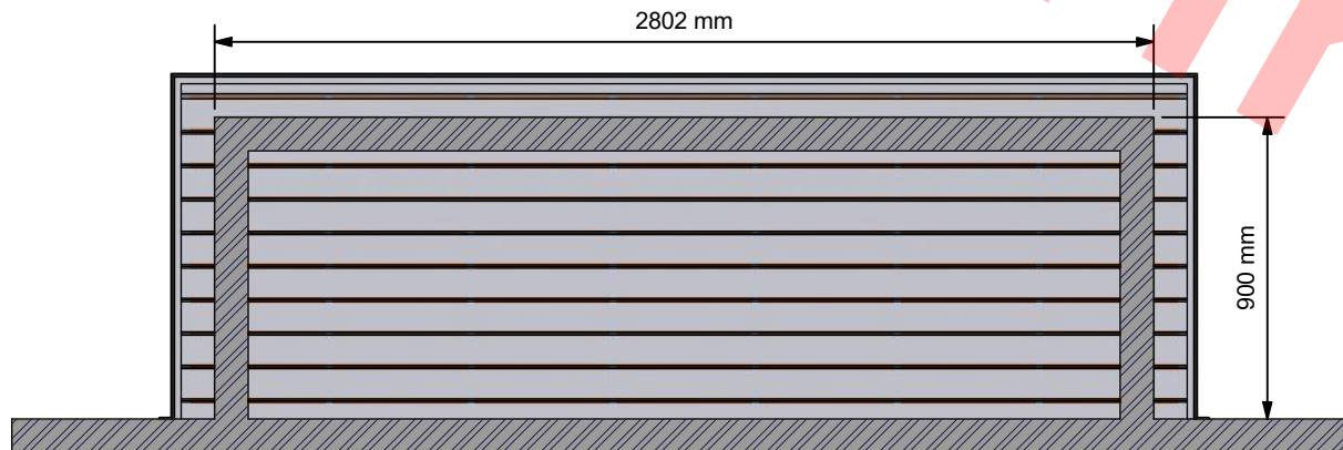
View On Underside Showing Bay Brickwork Dim's. ( 1:25 )
