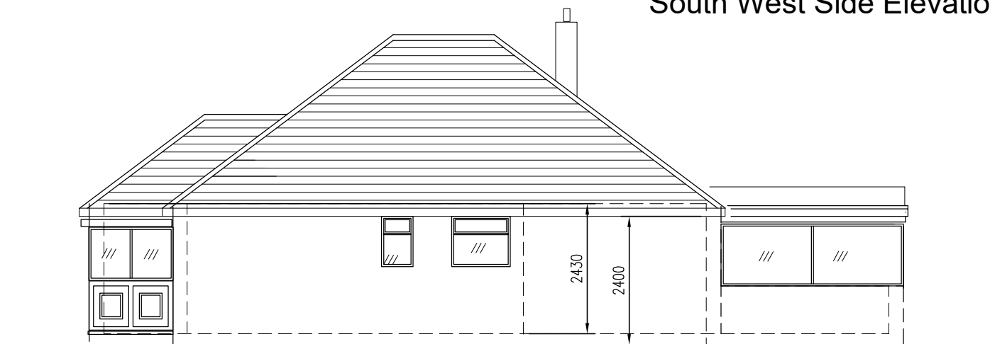
South West Side Elevation
