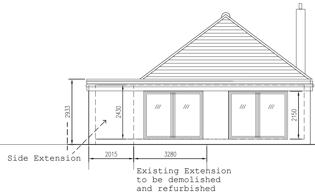
North West Rear Elevation
