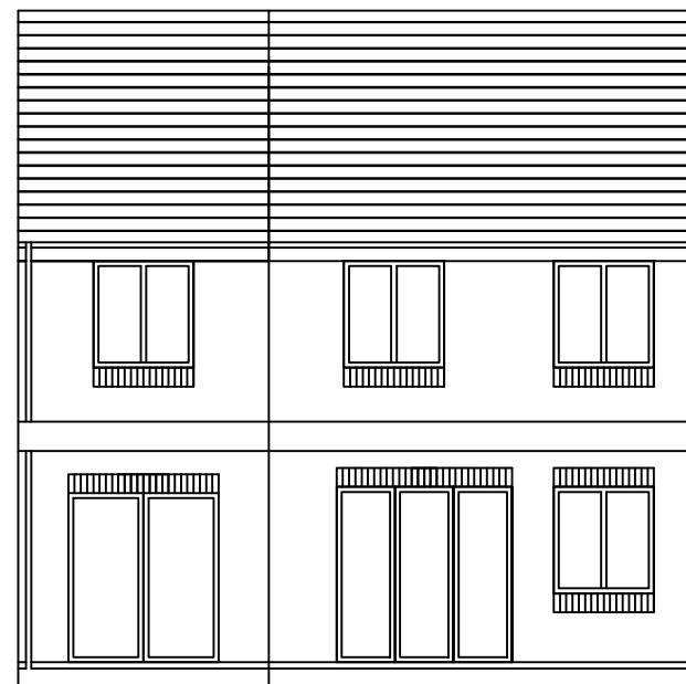
PROPOSED REAR
