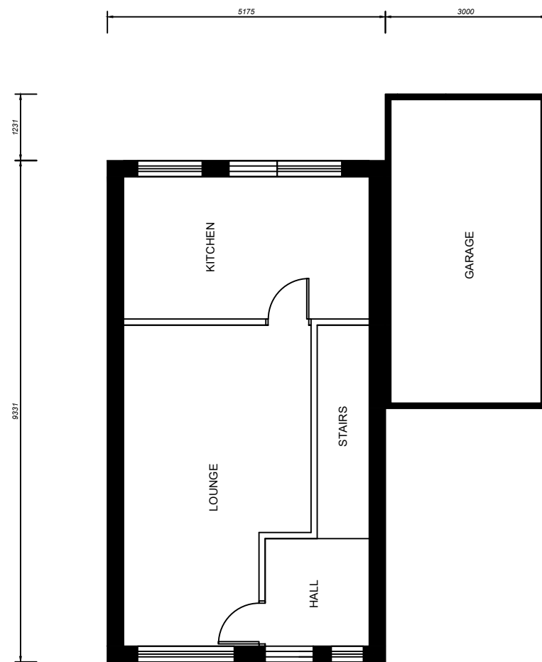
EXISTING GF
