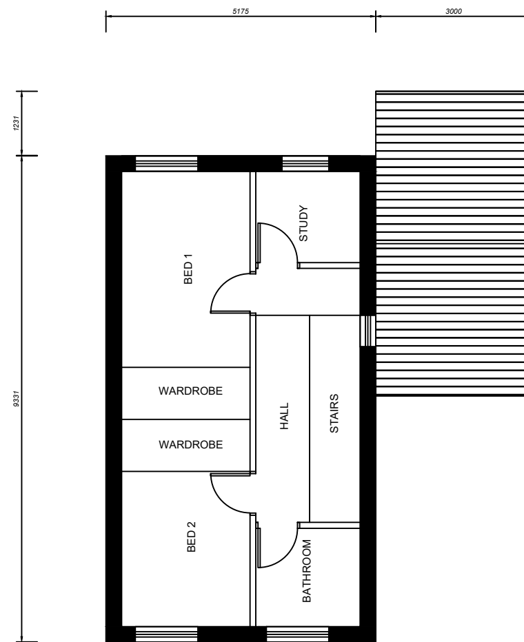
EXISTING FF
