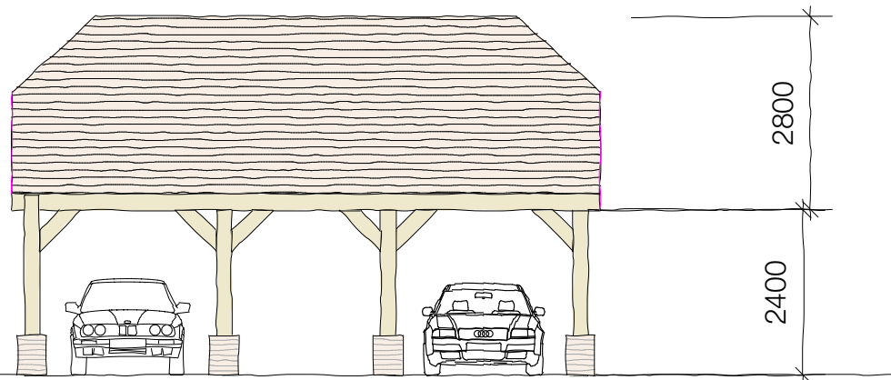
North Elevation
