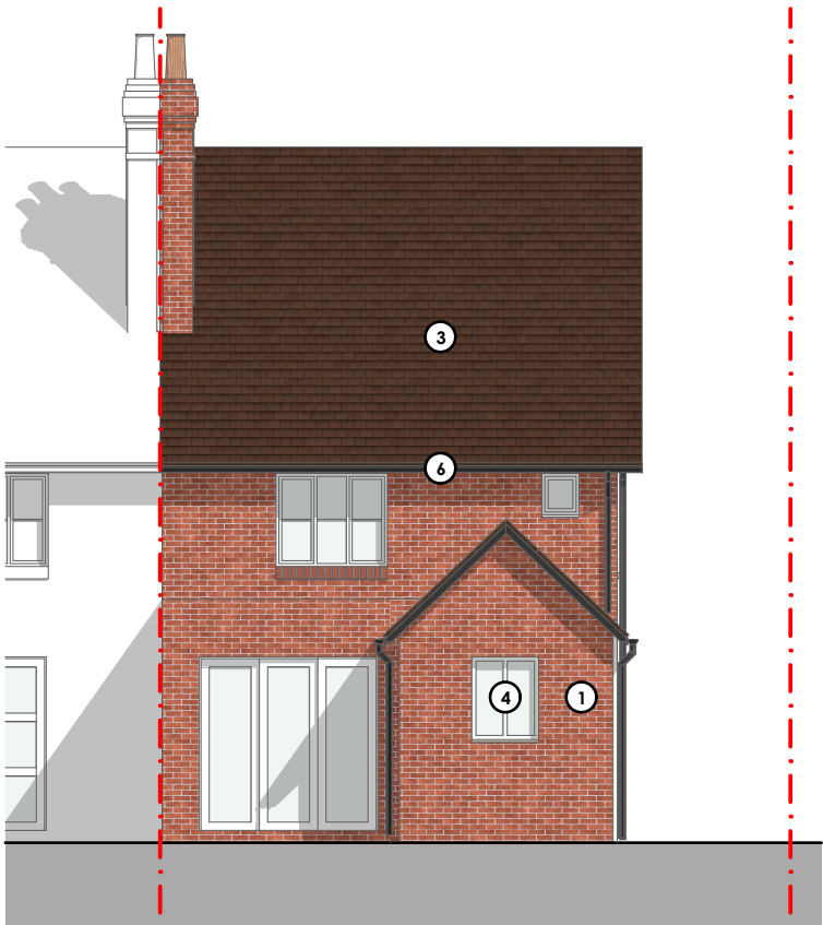
South (Rear) Elevation Existing
