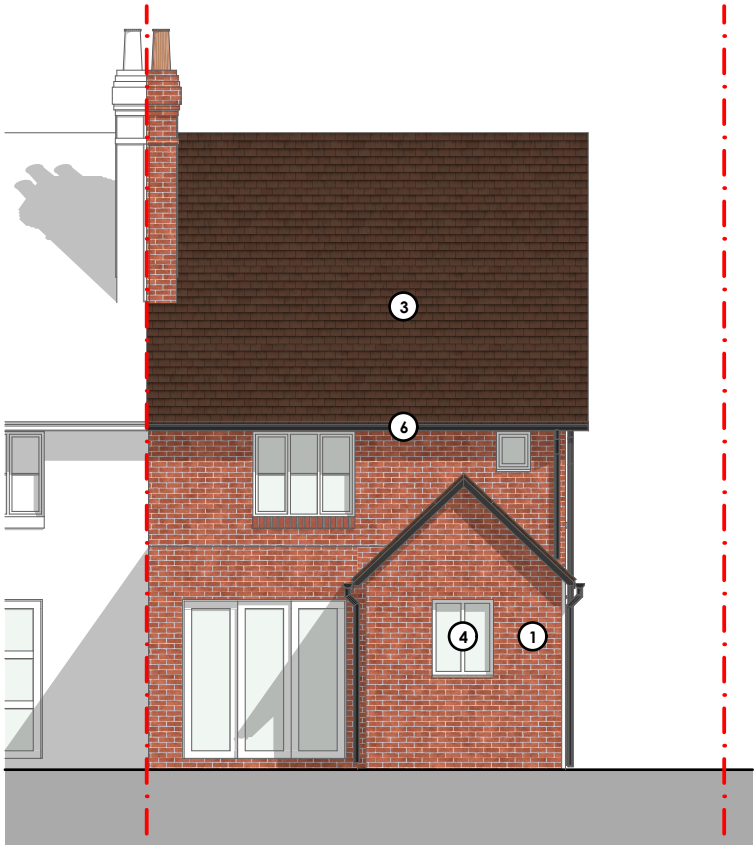
South (Rear) Elevation Proposed
