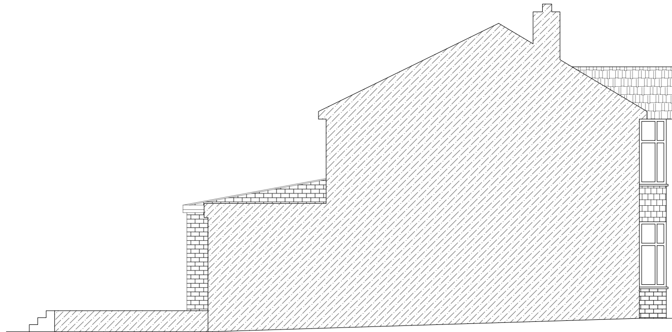
Existing South Elevation 1:100 @A3
