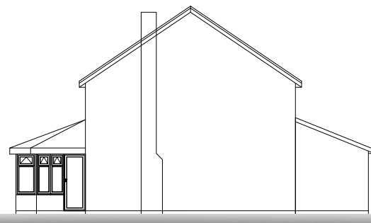
Existing Side Elevation scale: 1:100 @ A1, and 1:200 @ A3
