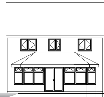
Existing Rear Elevation scale: 1:100 @ A1, and 1:200 @ A3 0 1:100 10m
