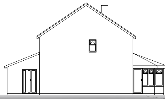
Existing Side Elevation scale: 1:100 @ A1, and 1:200 @ A3 0 1:100 10m
