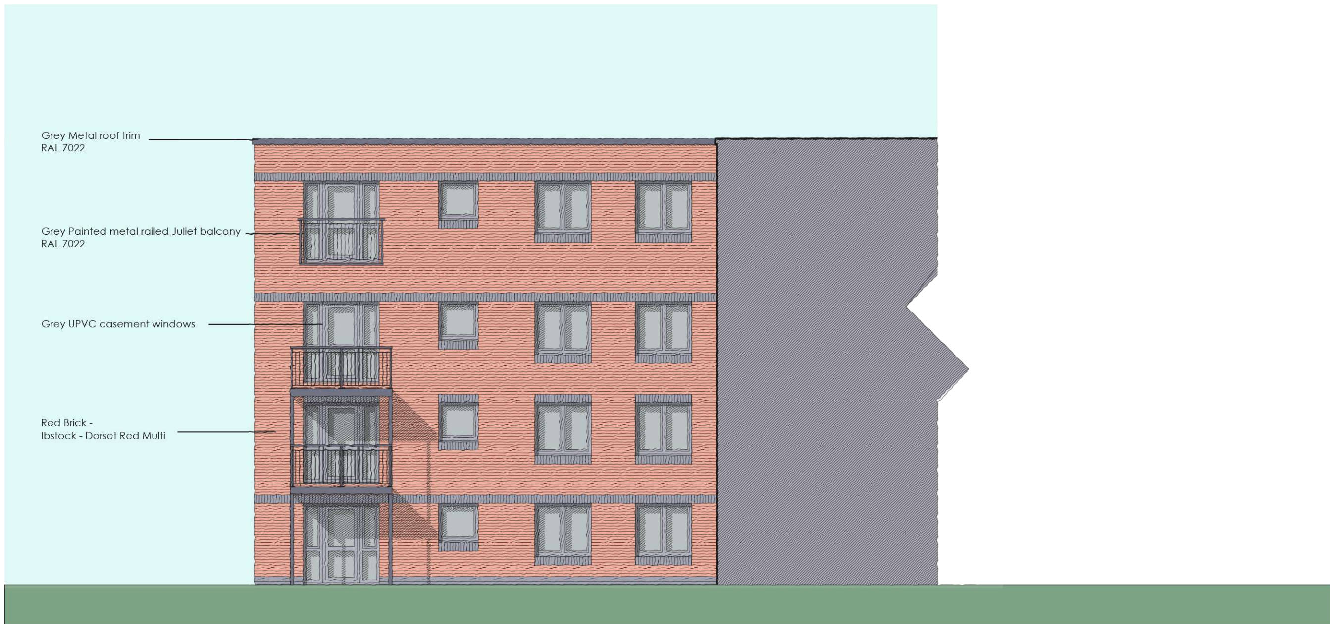
internal West Elevation - facing courtyard
