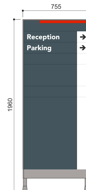
E Single-sided Freestanding Directional Sign 1:25 @ A3
