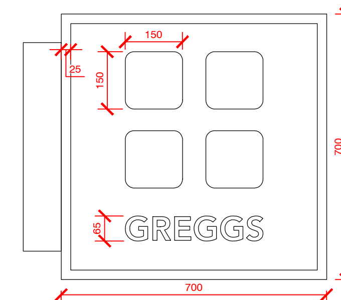
PROJECTING SIGN DETAIL (1:10)
