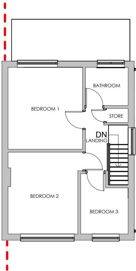
Existing First Floor Plan 1 : 100
