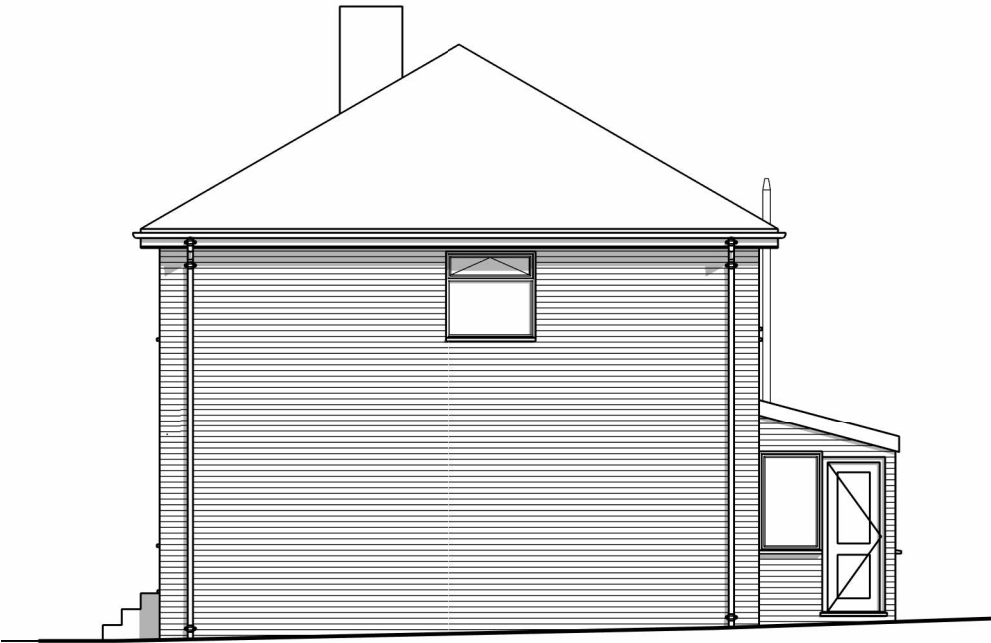
Existing East (Side) Elevation 1 : 100
