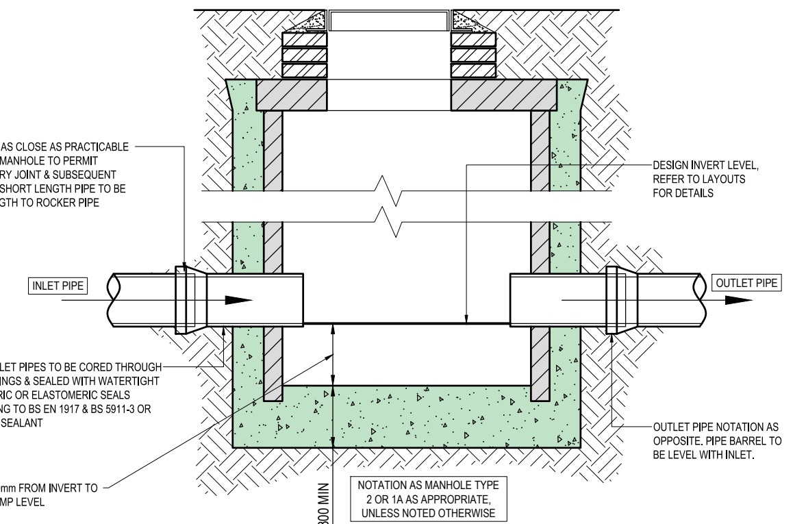
TYPE 2 CATCHPIT MANHOLE SECTION SIMILAR TO TYPE 2 / TYPE 1A MANHOLE ADDITIONAL REQUIREMENTS FOR CATCHPIT MANHOLE SHOWN (1:20 AT A1)
