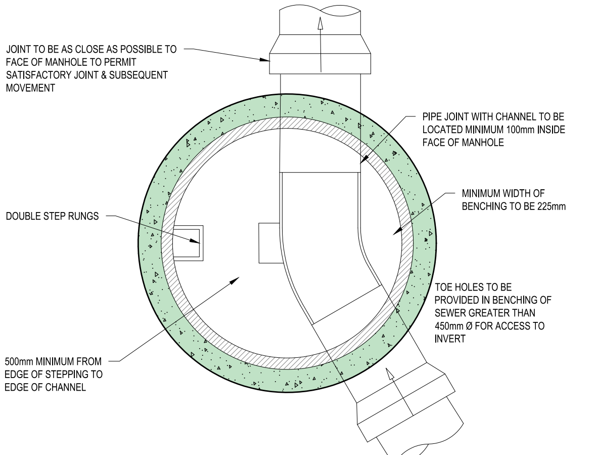
TYPICAL PCC MANHOLE DETAIL (TYPE 2) DEPTH FROM COVER LEVEL TO SOFFIT OF PIPE 2m TO 3m SCALE: 1:25
