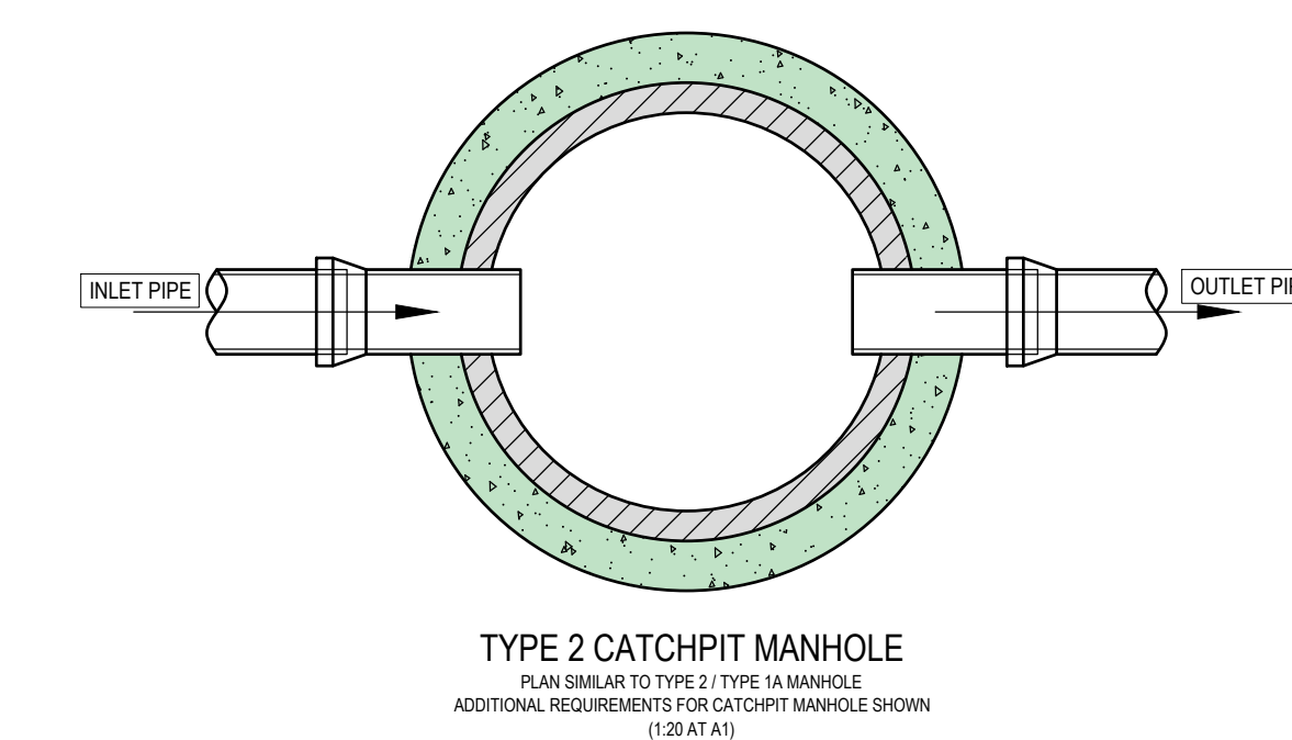
TYPE 2 CATCHPIT MANHOLE PLAN SIMILAR TO TYPE 2 / TYPE 1A MANHOLE ADDITIONAL REQUIREMENTS FOR CATCHPIT MANHOLE SHOWN (1:20 AT A1)
