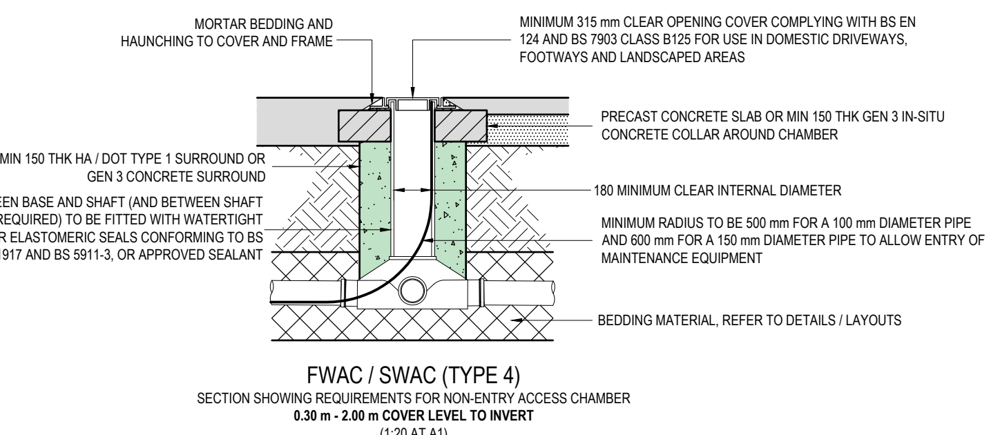
FWAC / SWAC (TYPE 4) SECTION SHOWING REQUIREMENTS FOR NON-ENTRY ACCESS CHAMBER 0.30m - 2.00m COVER LEVEL TO INVERT (1:20 AT A1)
