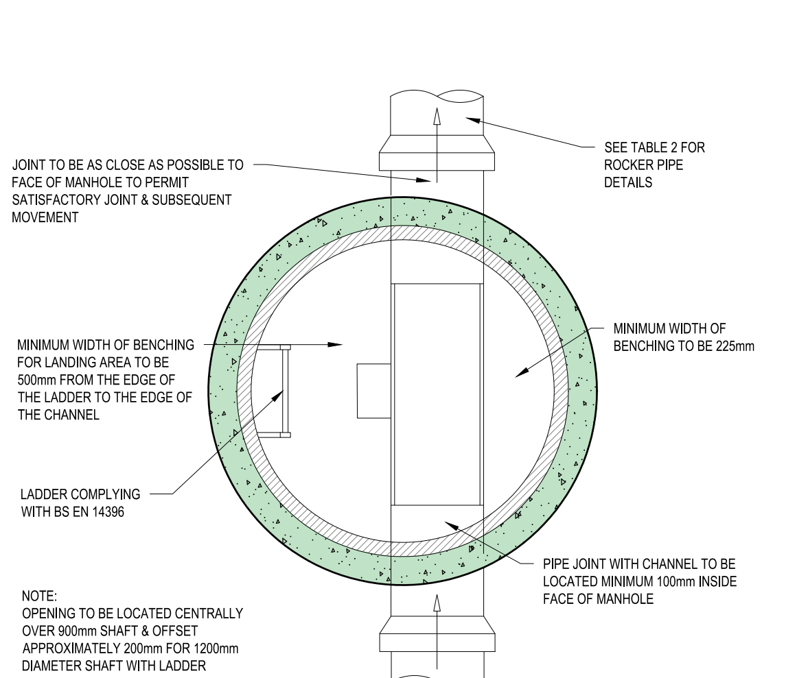
TYPICAL MANHOLE DETAIL (TYPE 1A) DEPTH FROM COVER LEVEL TO SOFFIT OF PIPE 3.0m to 6.0m SCALE: 1:25
