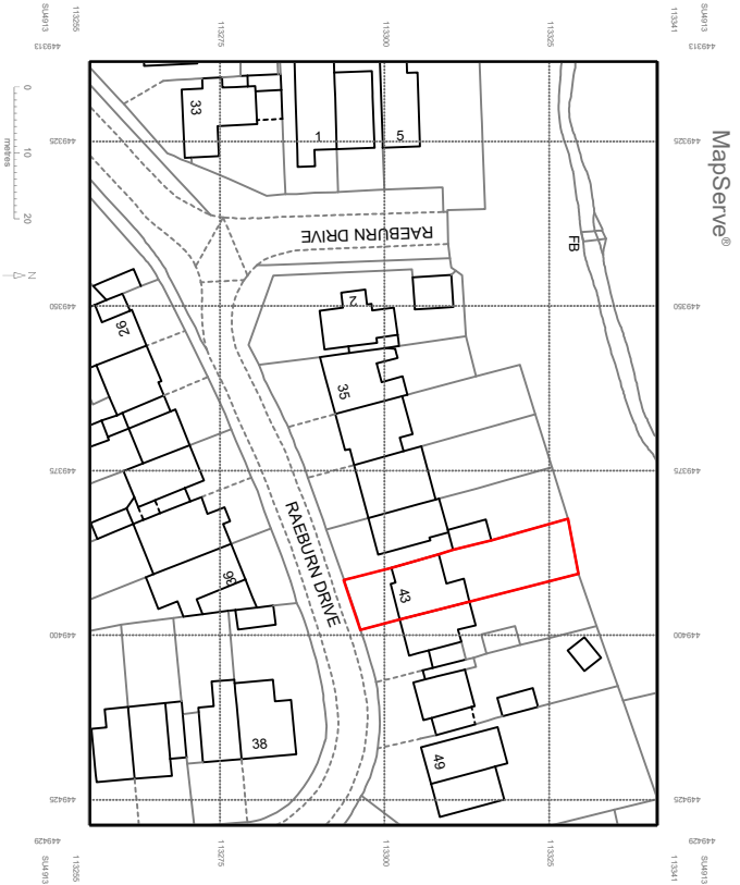
Site Location Plan I : 1250 @ A3
