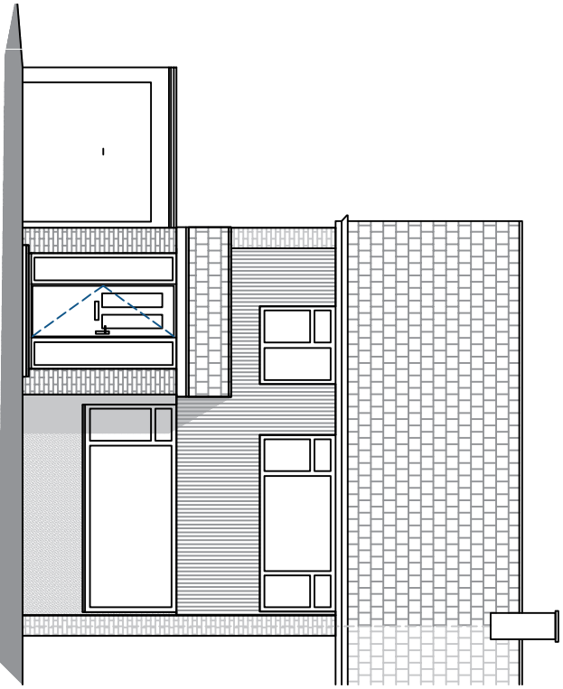
Proposed Front Elevation 1 : 100 @ A3
