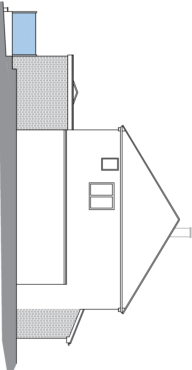
Proposed Side Elevation 1 : 100 @ A3
