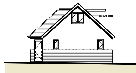
Front (South East) Elevation
