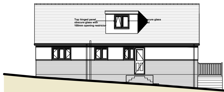
Side (North East) Elevation
