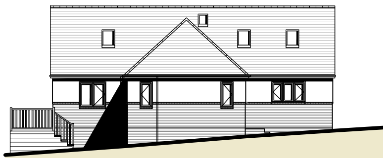
Side (South West) Elevation
